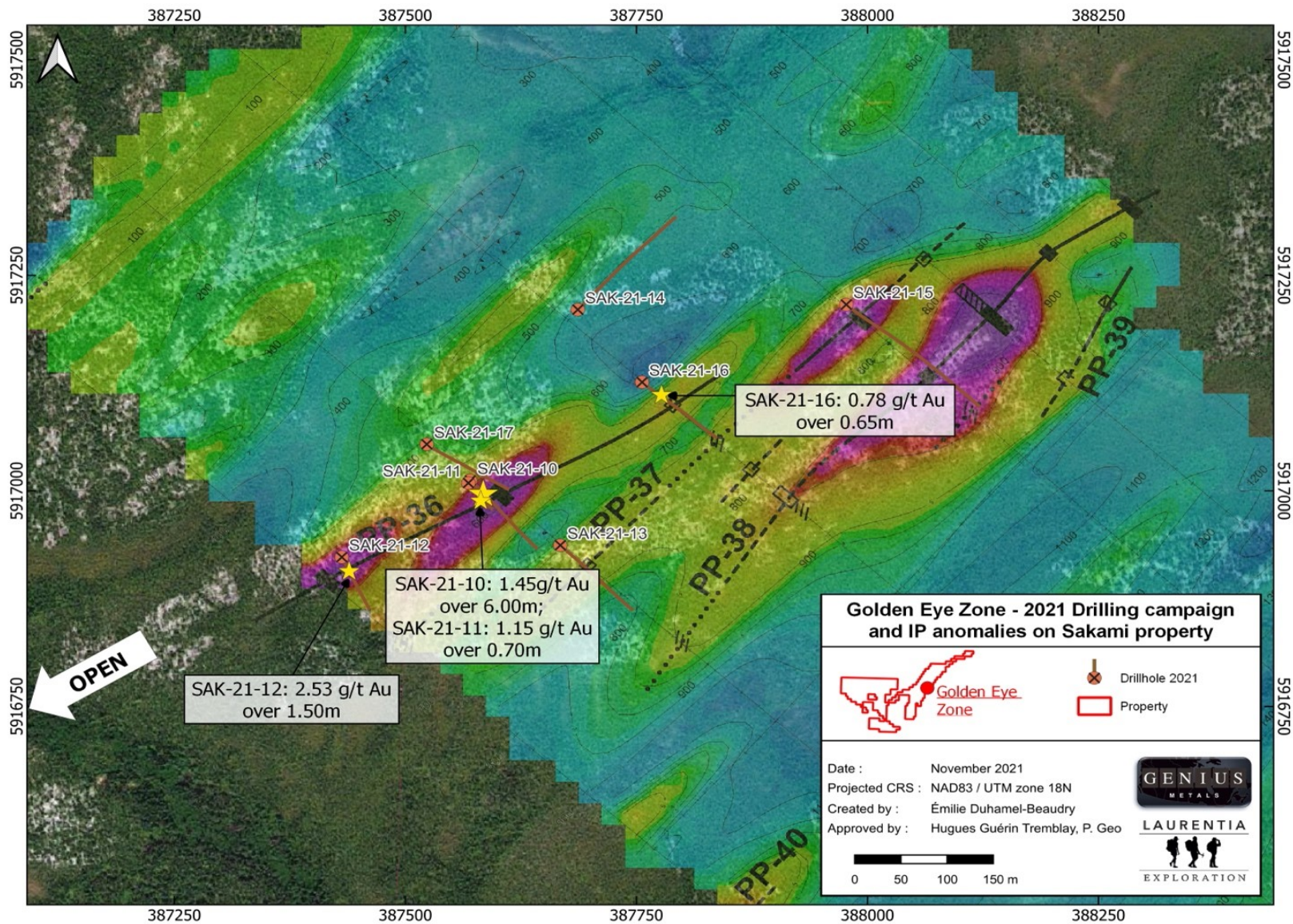
Figure 1. Chargeability contour map showing de main assay results from Genius Metals 2021 drilling campaign on the Golden Eye prospect, Sakami property
