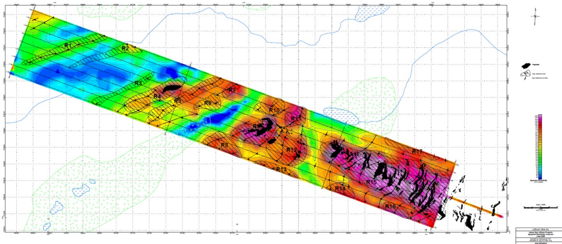
Figure 2. Contour map, apparent resistivity, Lithium One (2008)
